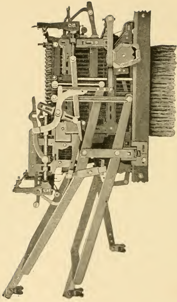
CROSS BORDER DOUBLE-LIFT JACQUARD MACHINE
